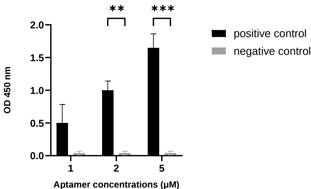
Direct ELASA with thiolated aptamer
